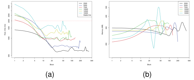
Fig. 6. Scalability analysis for the AG-cl-I data stream with respect to different data block size. (a) Processing time. (b) Memory consumption.
